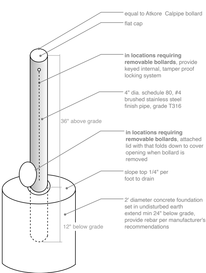
Typical Bollard (non-removable or removable)
