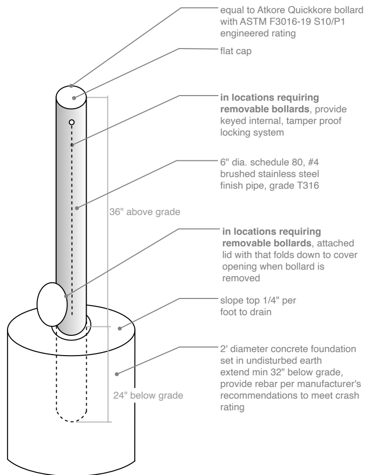
Crash Rated Bollard (non-removable or removable)
