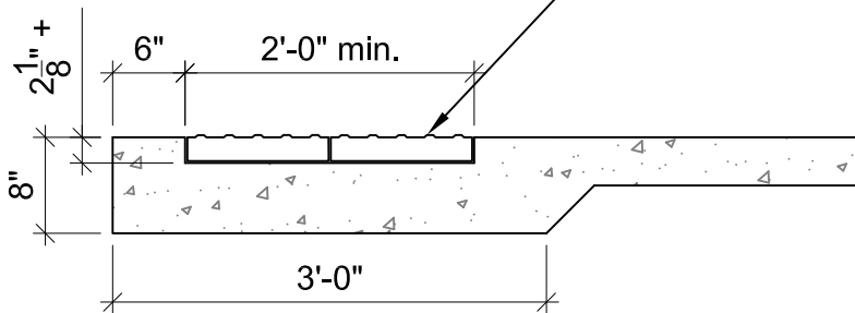
2 SECTION NTS
