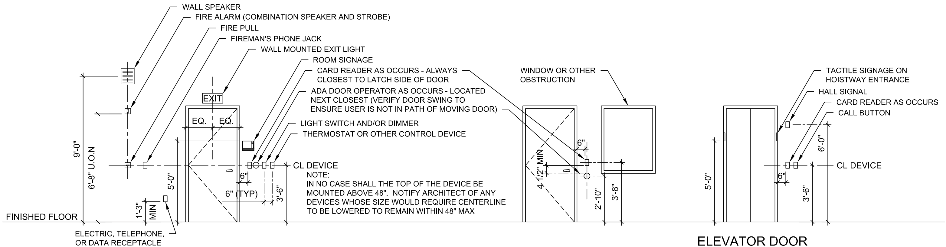
OPTION #1 - SIDE BY SIDE (PREFERRED INSTALLATION METHOD)
